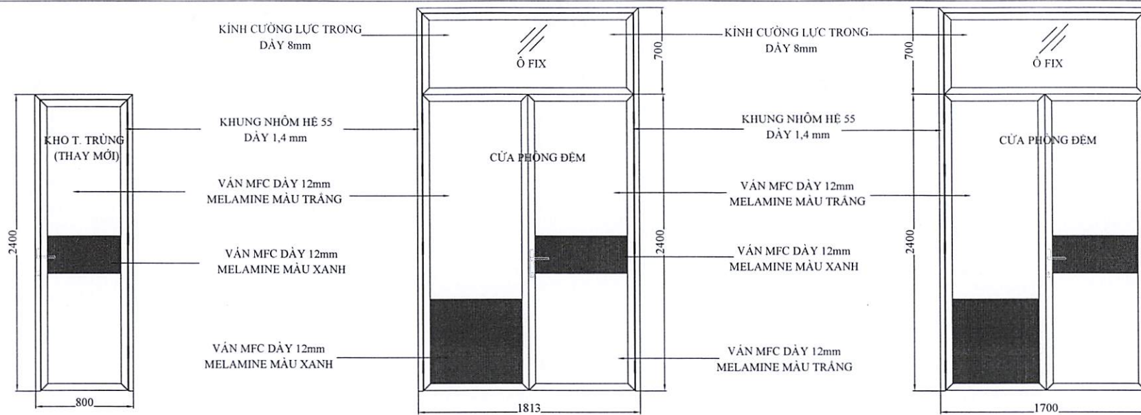
CỬA: MD - 13, SL: 1 BỘ, TL 1/40
